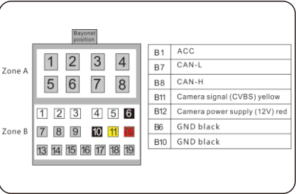
2.Interface definition diagram
