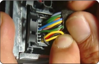
3.Insert the rear view extension cable socket into the main unit power supply (as shown in the figure below)
